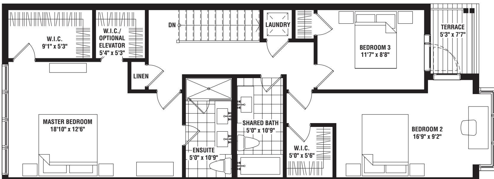
Second Floor
