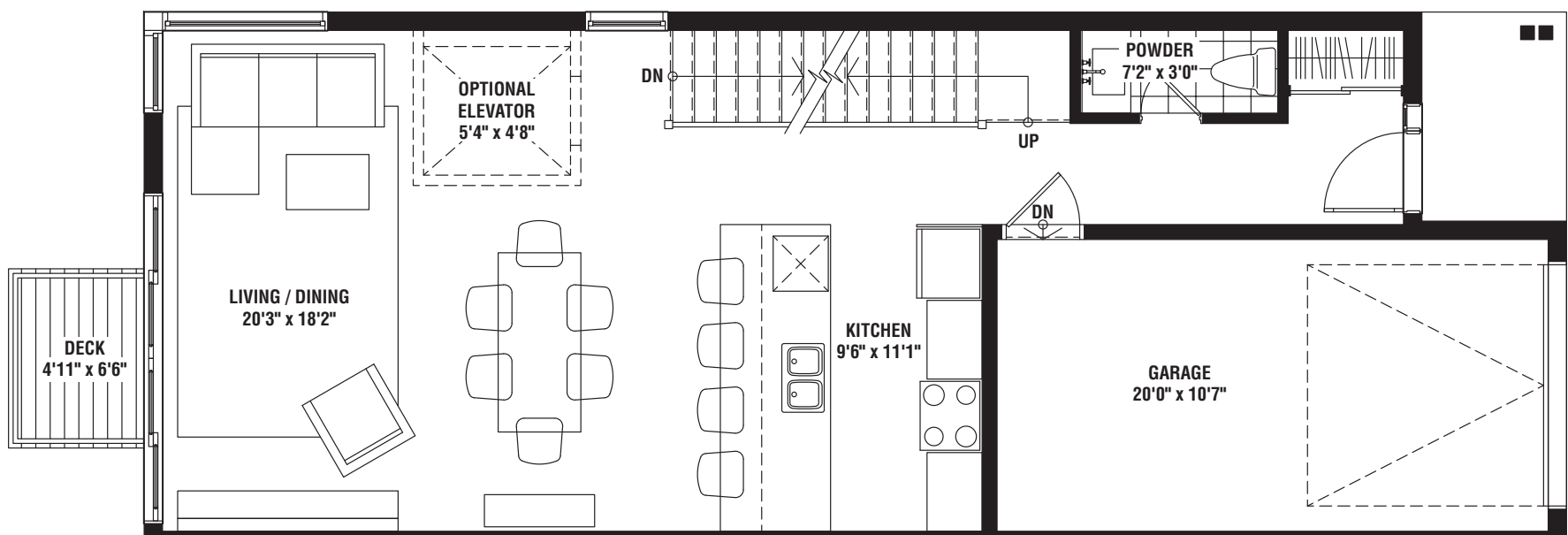
Ground Floor (End)
