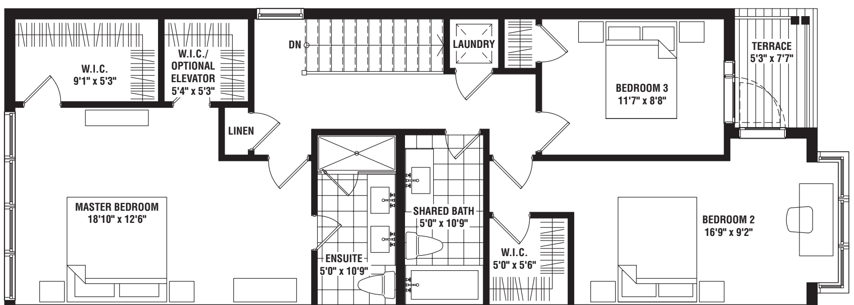
Second Floor (End)
