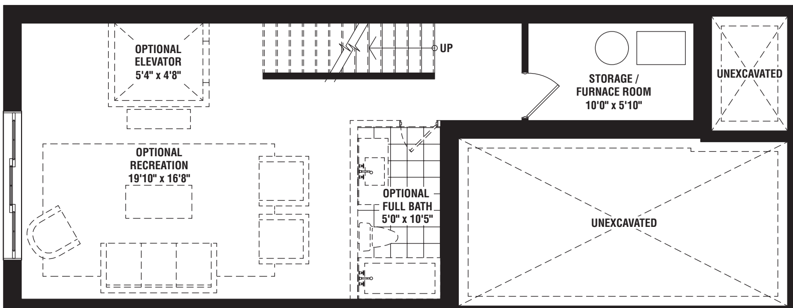
Basement
